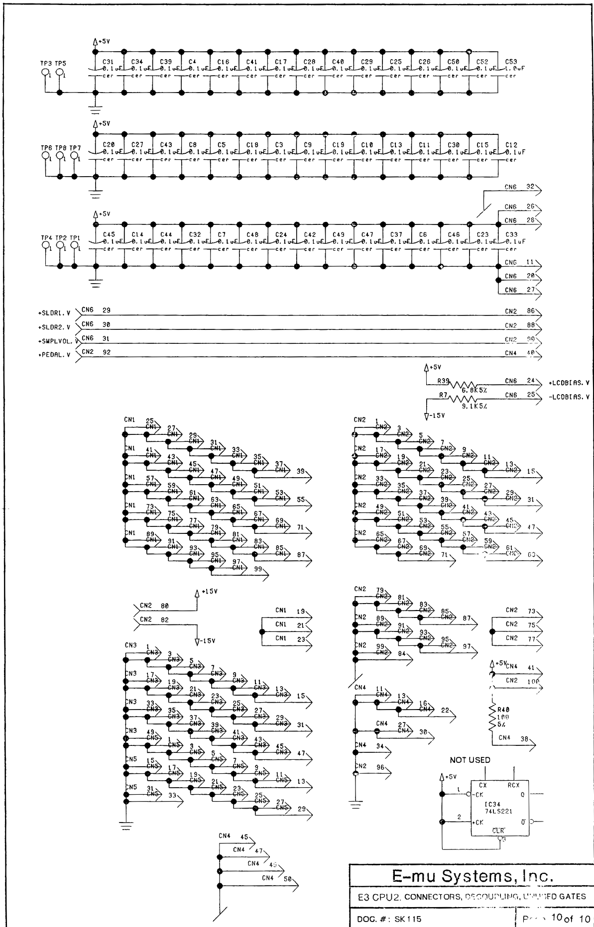
CPU Board (CPU2) — SK115 sheet 10 of 10: CPU2: Connectors, Decoupling, Unused Gates.
