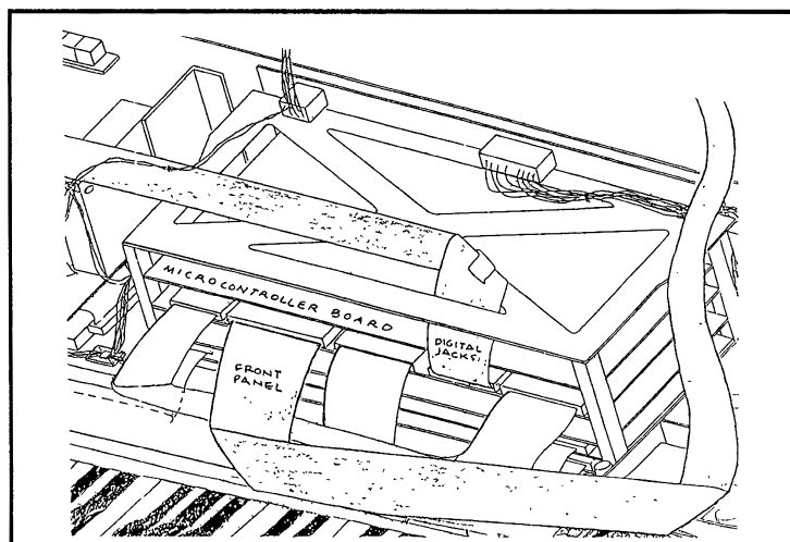
Routing of the digital jack and front panel ribbon cables.
