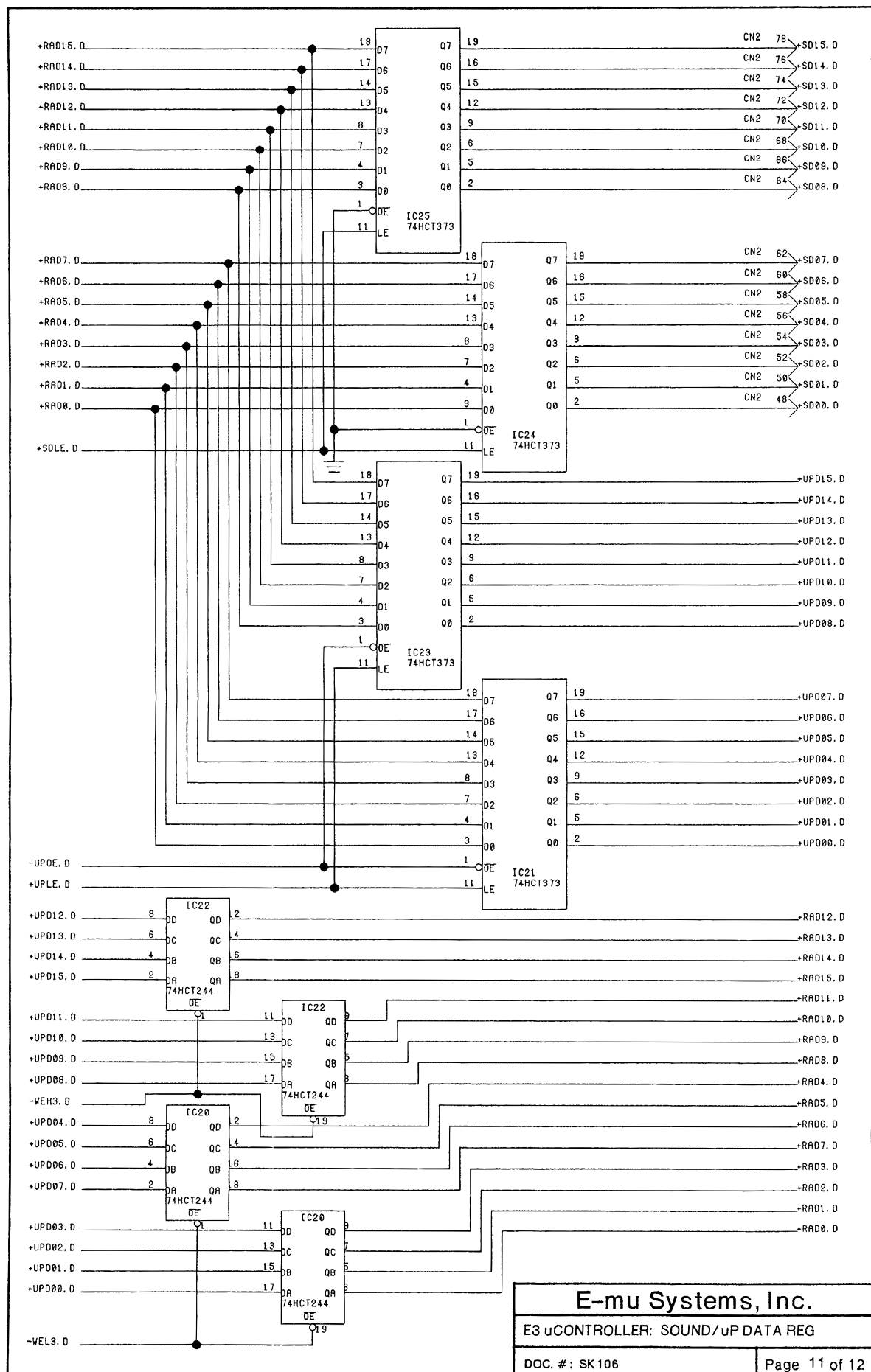
Microcontroller Board — SK106 sheet 11 of 12: uController: Sound/uP Data Reg.
