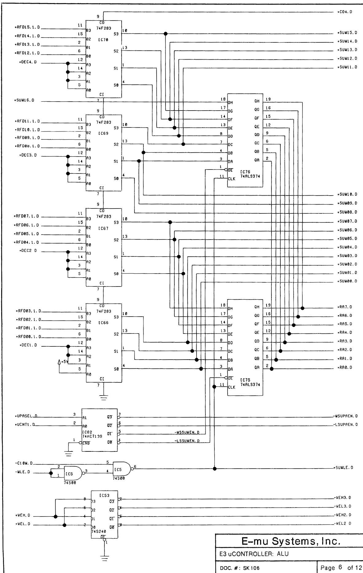
Microcontroller Board — SK106 sheet 6 of 12: uController: ALU.
