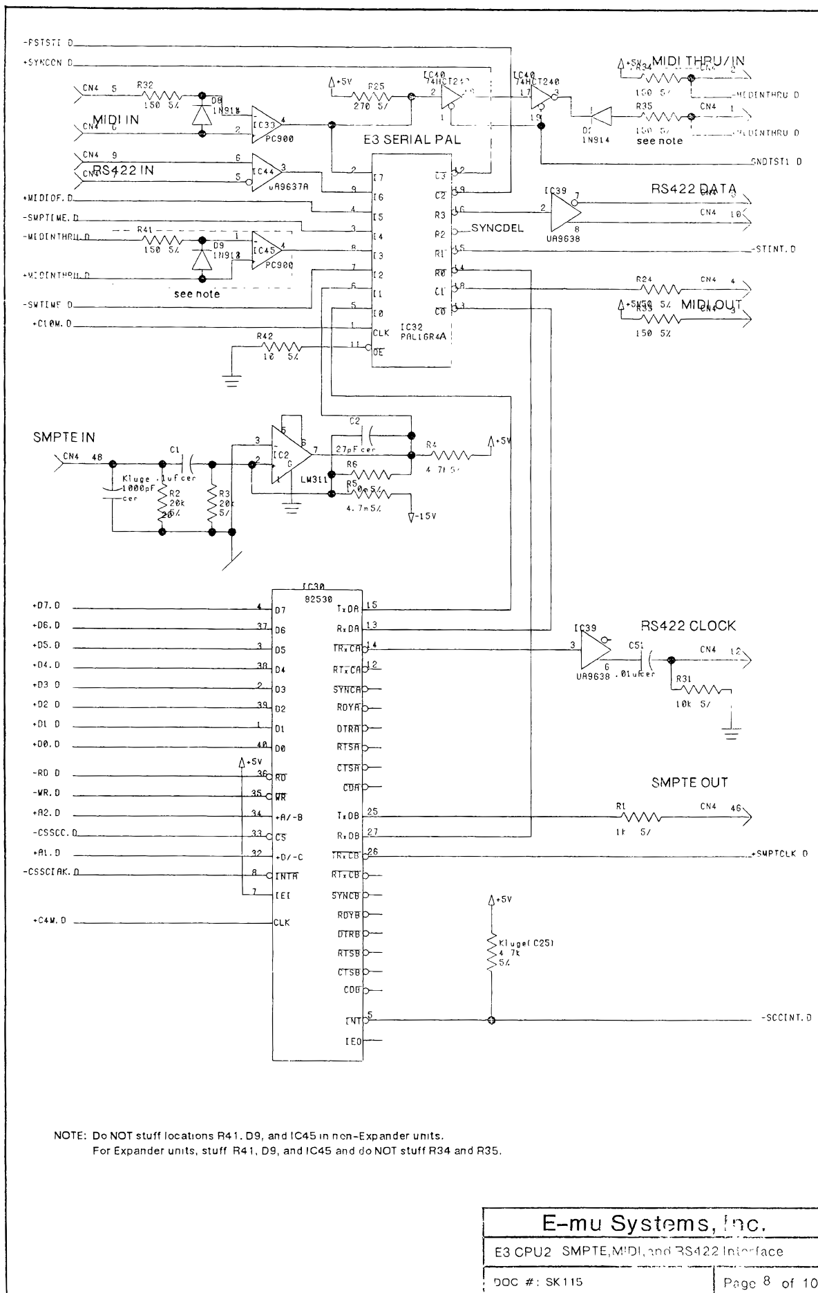
CPU Board (CPU2) — SK115 sheet 8 of 10: CPU2: SMPTE, MIDI and RS422 Interface.
