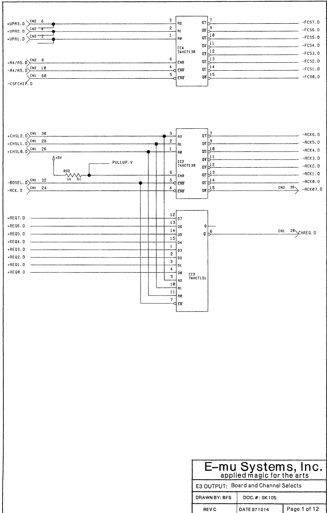
Output Board — SK105 sheet 1 of 12: Output: Board and Channel Selects.
