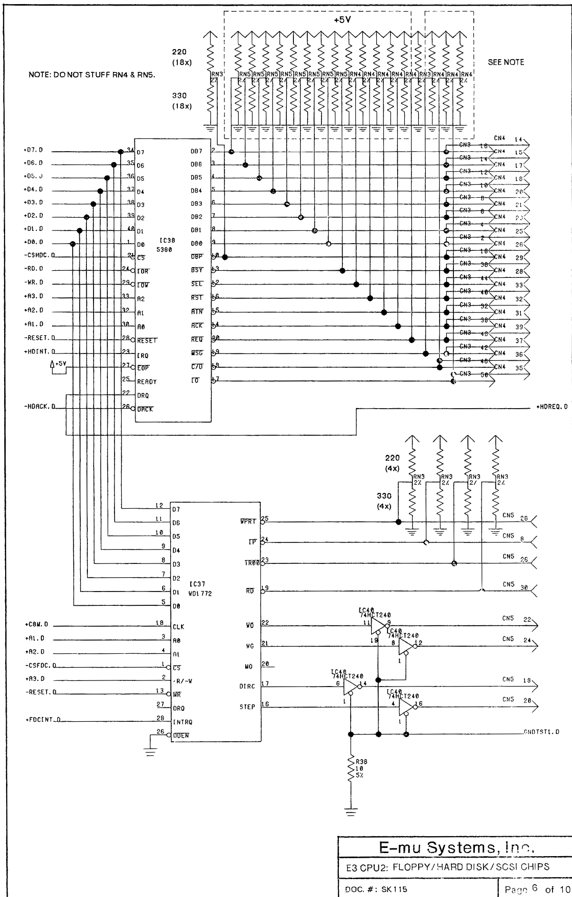
CPU Board (CPU2) — SK115 sheet 6 of 10: CPU2: Floppy/Hard Disk/SCSI Chips.
