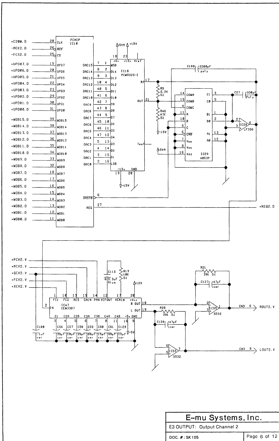
Output Board — SK105 sheet 6 of 12: Output: Output Channel 2.
