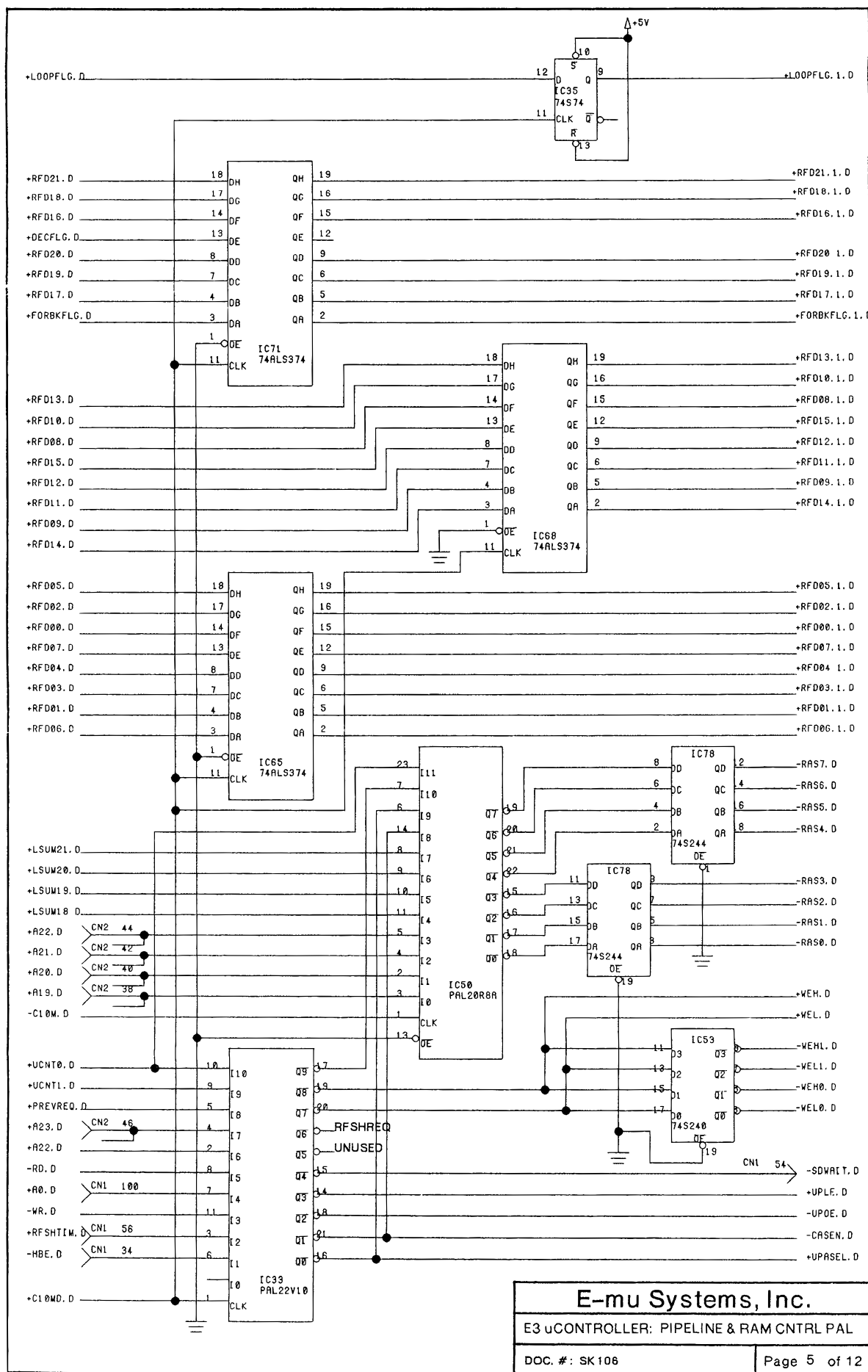
Microcontroller Board — SK106 sheet 5 of 12: uController: Pipeline & RAM Cntrl PAL.
