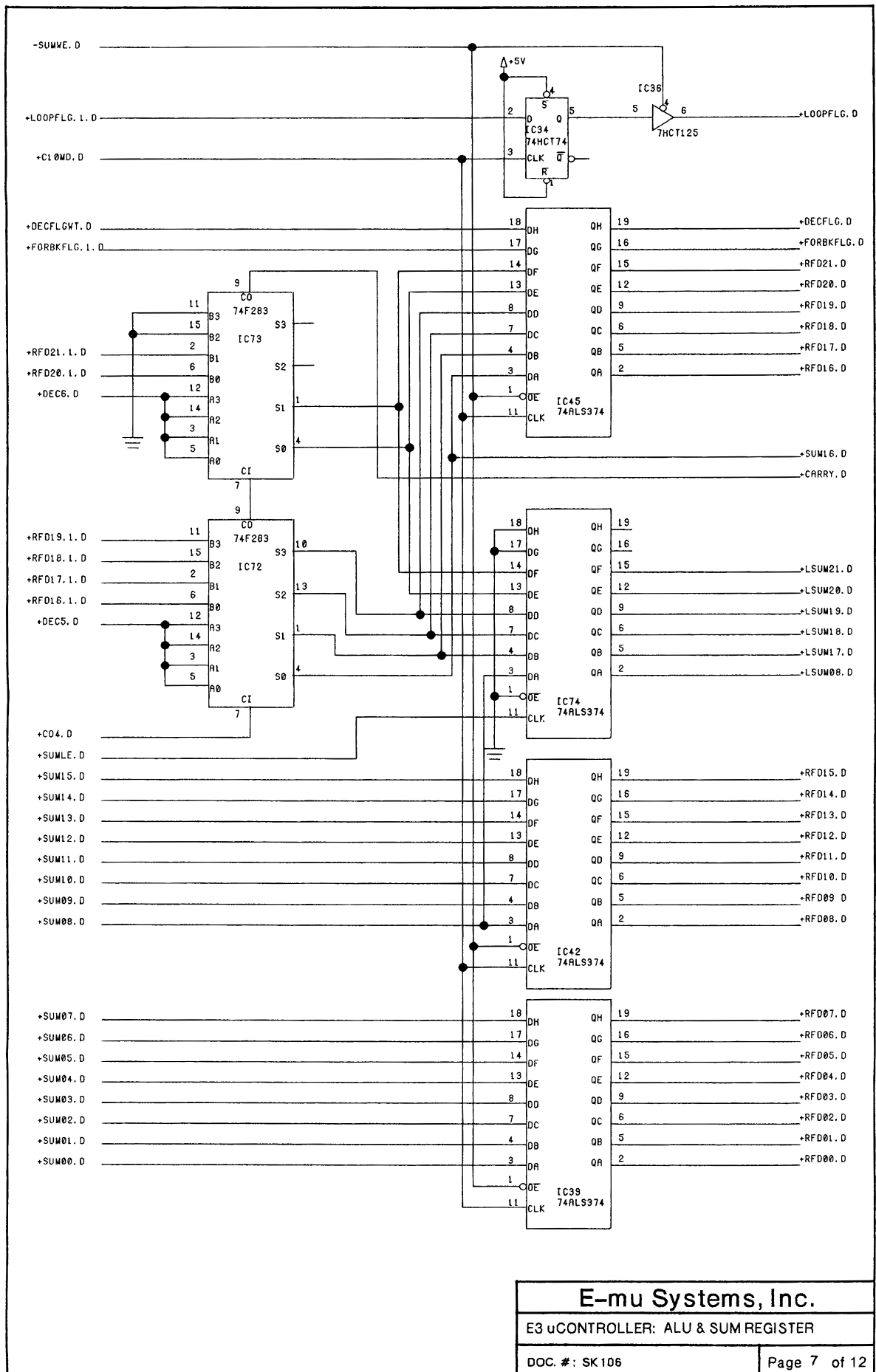
Microcontroller Board — SK106 sheet 7 of 12: uController: ALU & Sum Register.
