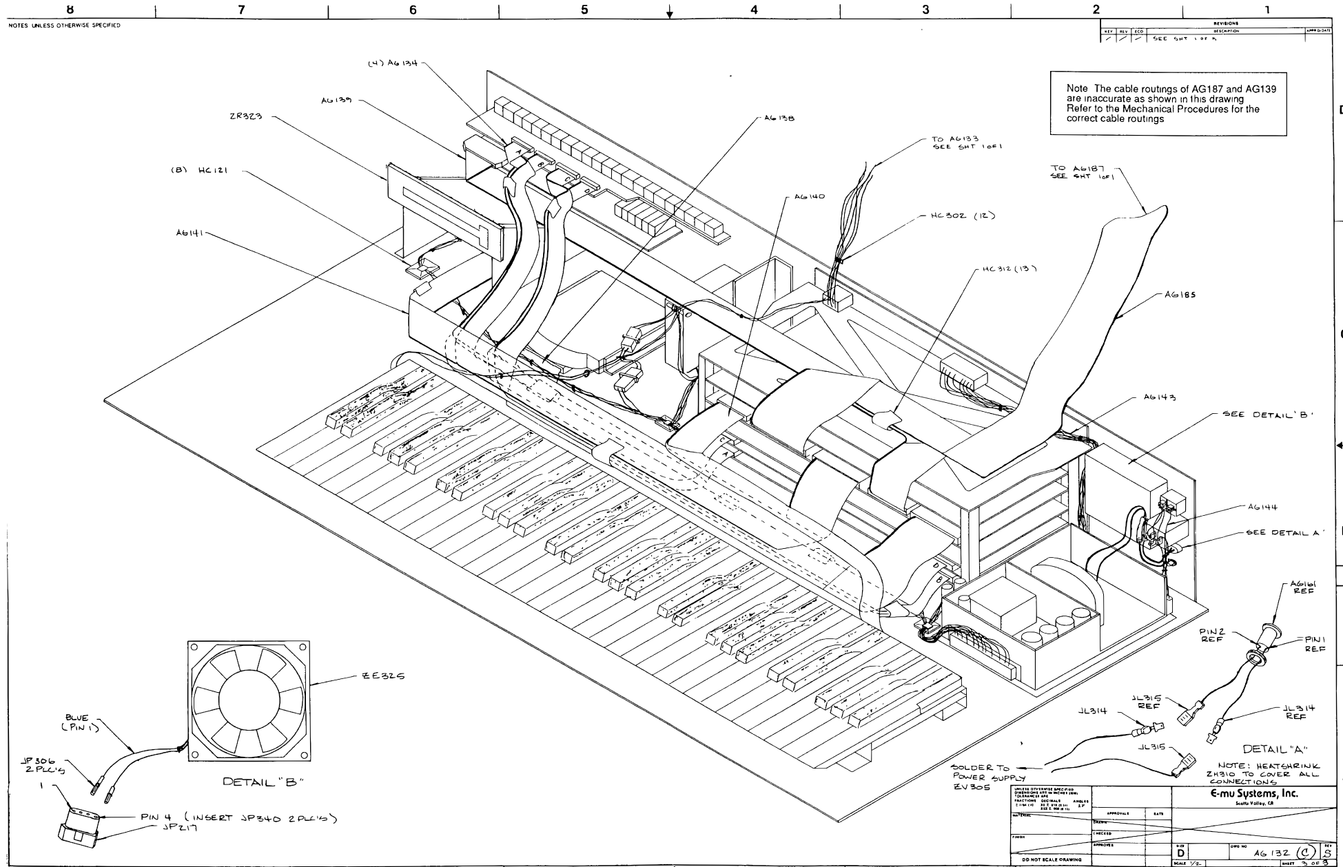
Drawing AG132, sheet 3 of 3 — Final assembly, keyboard 4 MEG E-3, Rev S.
