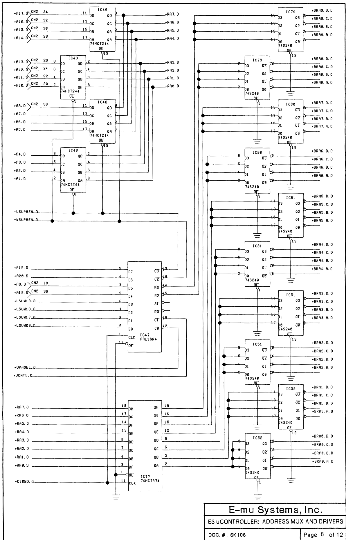
Microcontroller Board — SK106 sheet 8 of 12: uController: Address Mux and Drivers.
