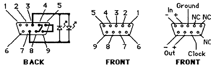
RS-422 test plug, back (wiring) and front views. Pinout: 3 Ground, 4 In+, 5 In-, 7 Clock, 8 Out+, 9 Out-; pins 1, 2 and 6 NC. Out is looped back to In (pins 4-8 and 5-9) and the two LEDs show that the clock is running.
