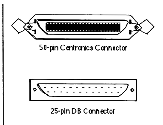
The two SCSI cable connector types: 50-pin Centronics and 25-pin DB.
