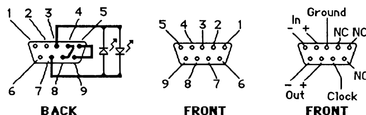
RS-422 test plug (same drawing as in the Functional Test Procedure chapter).
