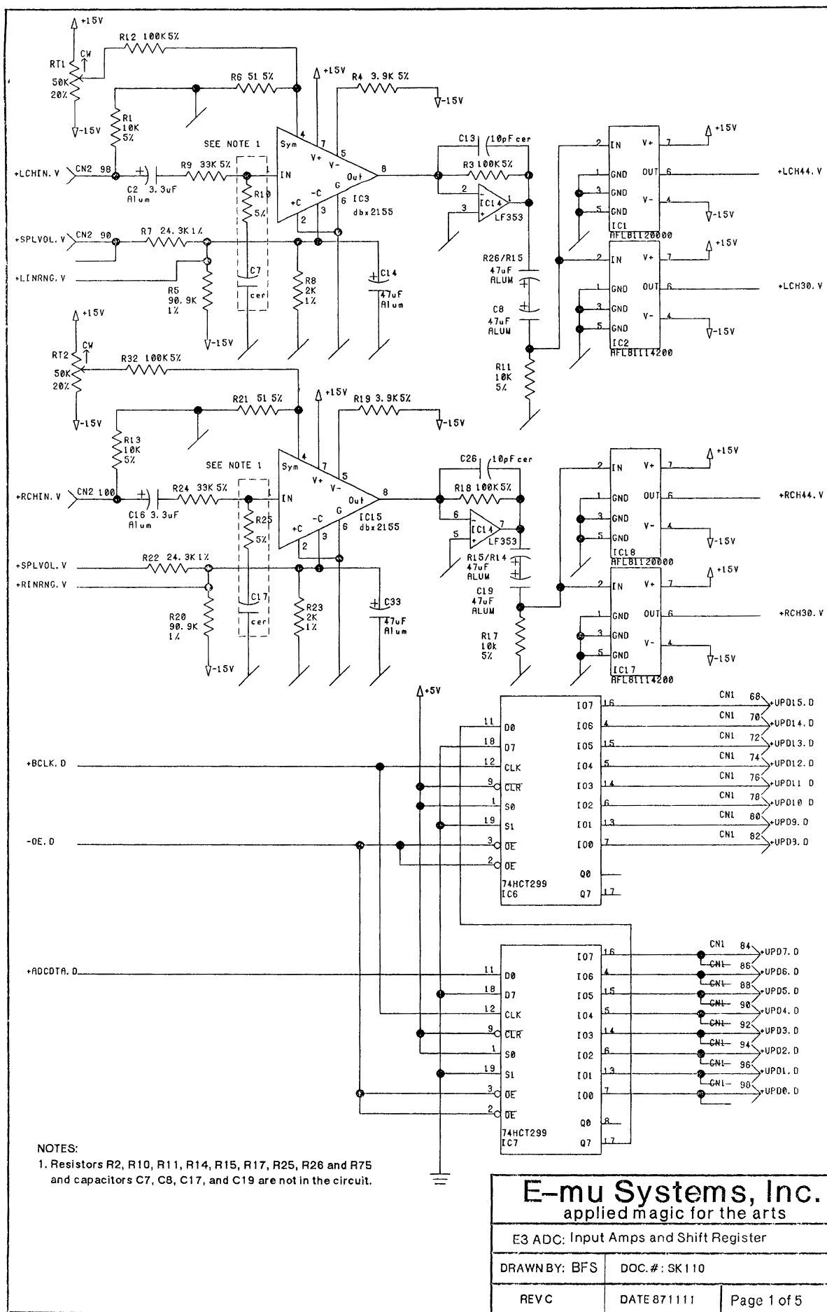
ADC Board — SK110 sheet 1 of 5: ADC: Input Amps and Shift Register.
