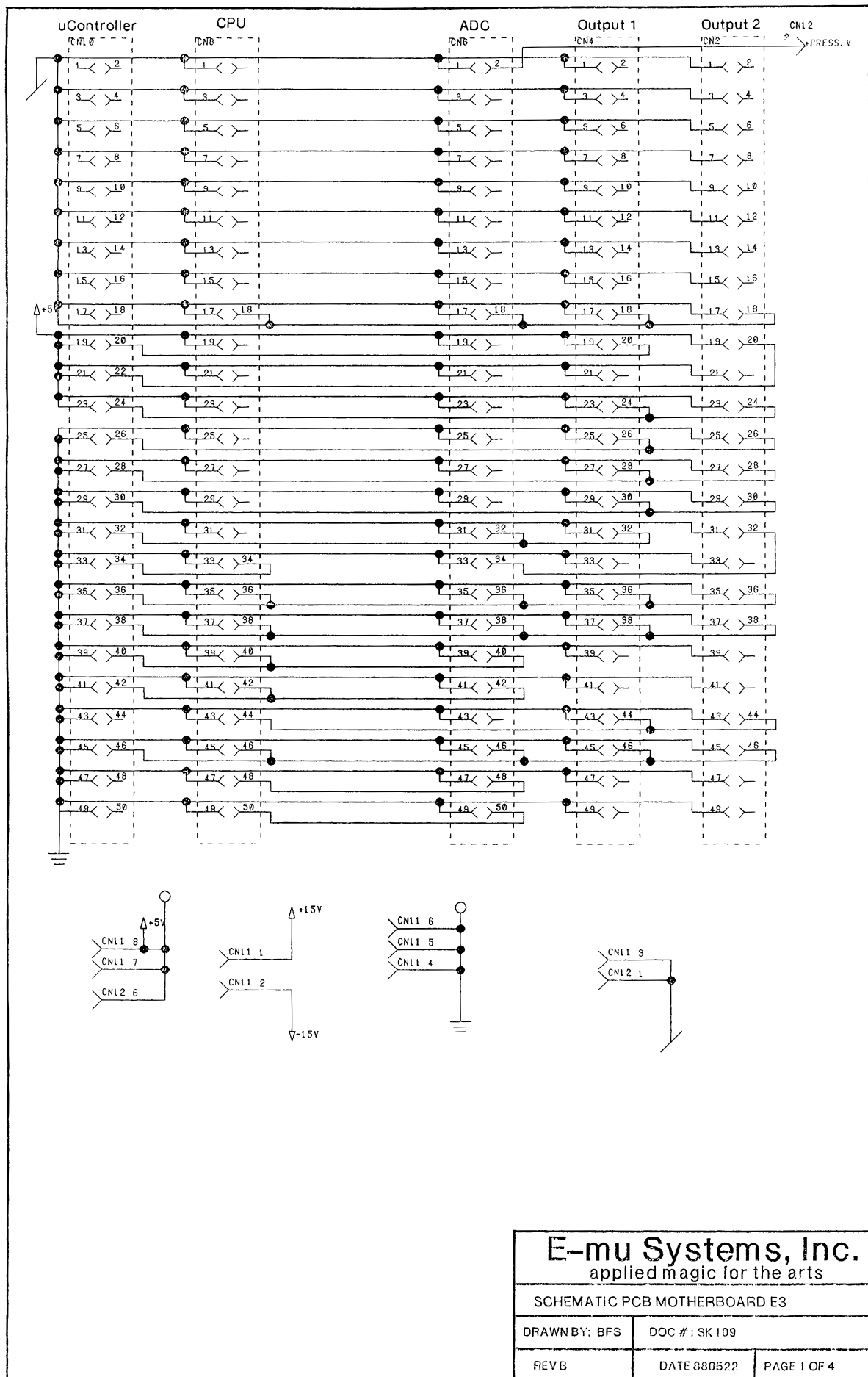
Motherboard — SK109 sheet 1 of 4: Motherboard.
