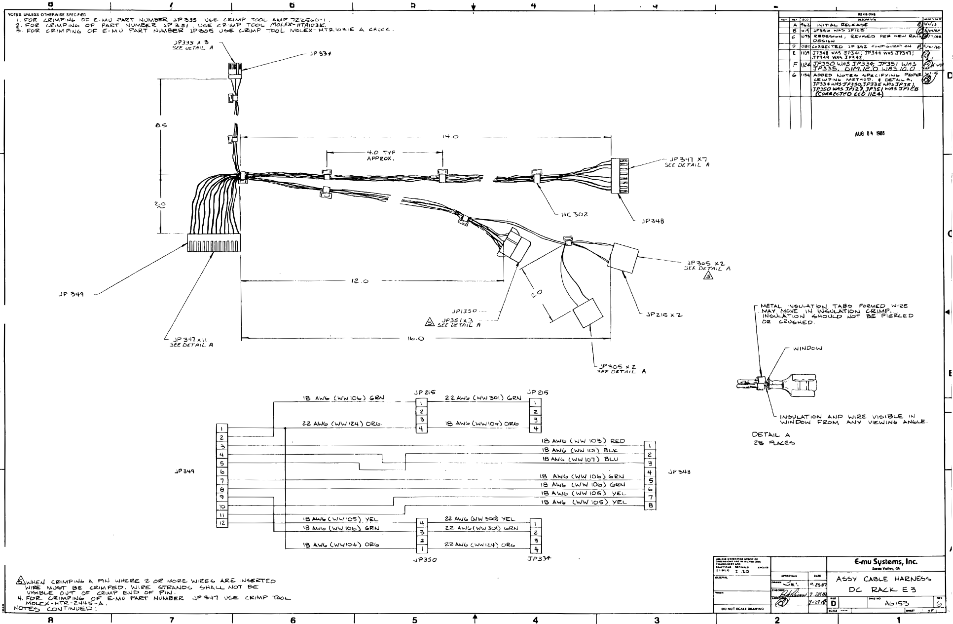
Drawing AG153 Rev G — Assy, cable harness, DC, rack, E3.
