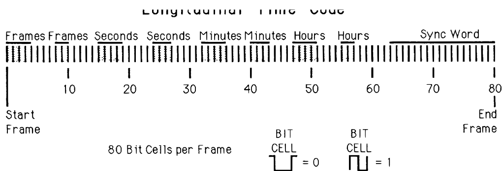
Longitudinal Time Code: one frame of 80 bit cells. A cell with no transition in its middle is a 0, a cell with a transition is a 1.
