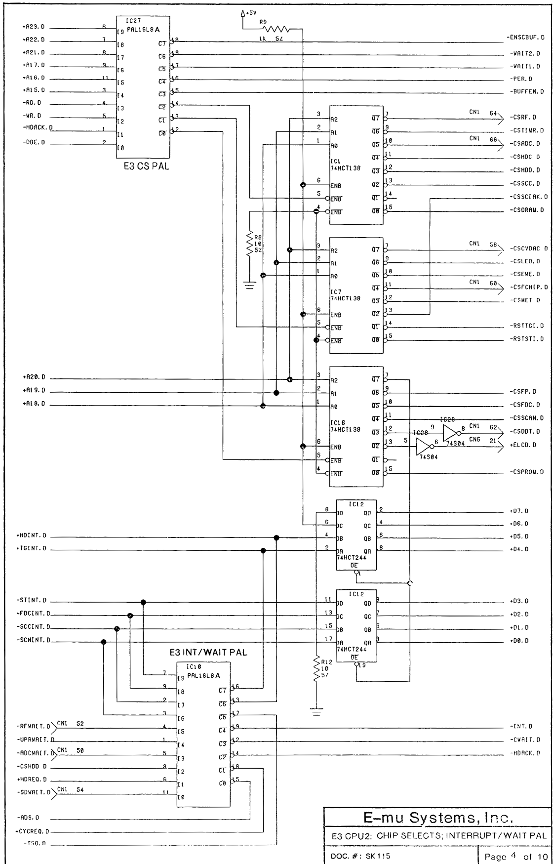
CPU Board (CPU2) — SK115 sheet 4 of 10: CPU2: Chip Selects, Interrupt/Wait PAL.
