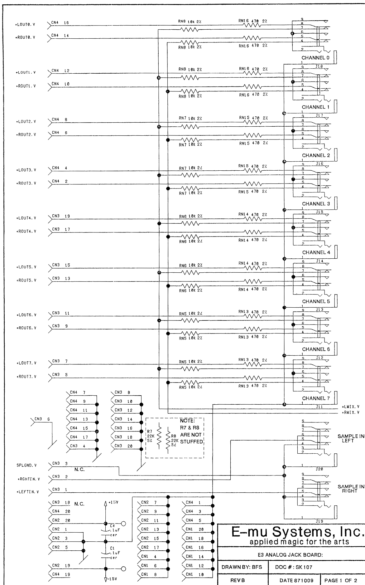
Analog Jack Board — SK107 sheet 1 of 2: Analog Jack Board.
