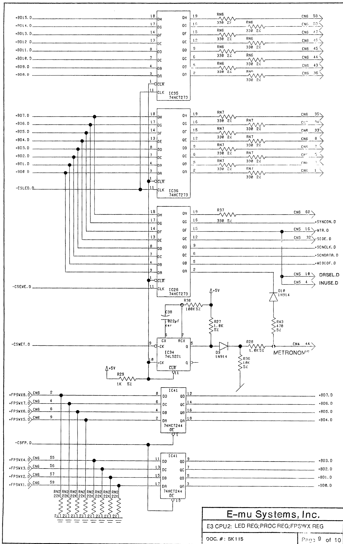
CPU Board (CPU2) — SK115 sheet 9 of 10: CPU2: LED Reg, Proc Reg, FPSWX Reg.
