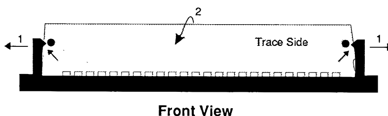
SIMM removal, front view: (1) push the end tabs outward, (2) tilt the SIMM toward you.
