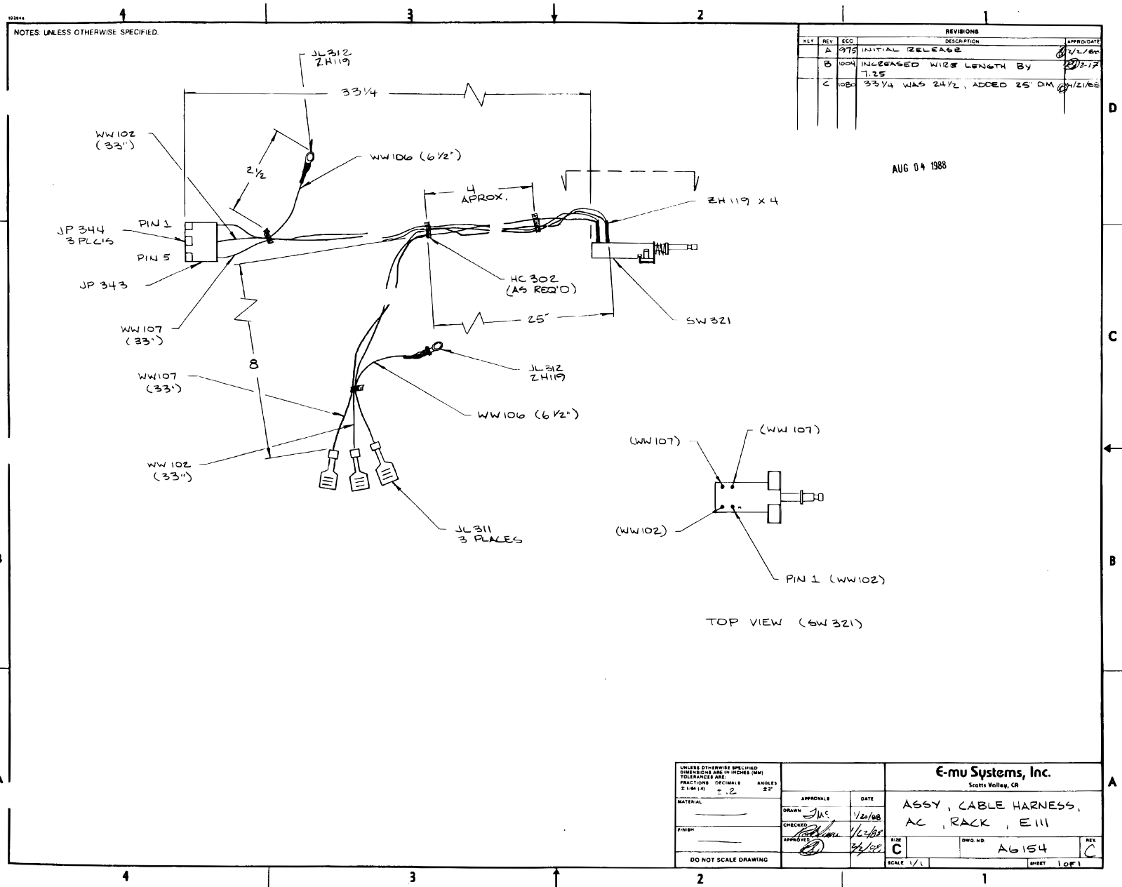
Drawing AG154 Rev C — Assy, cable harness, AC, rack, EIII.
