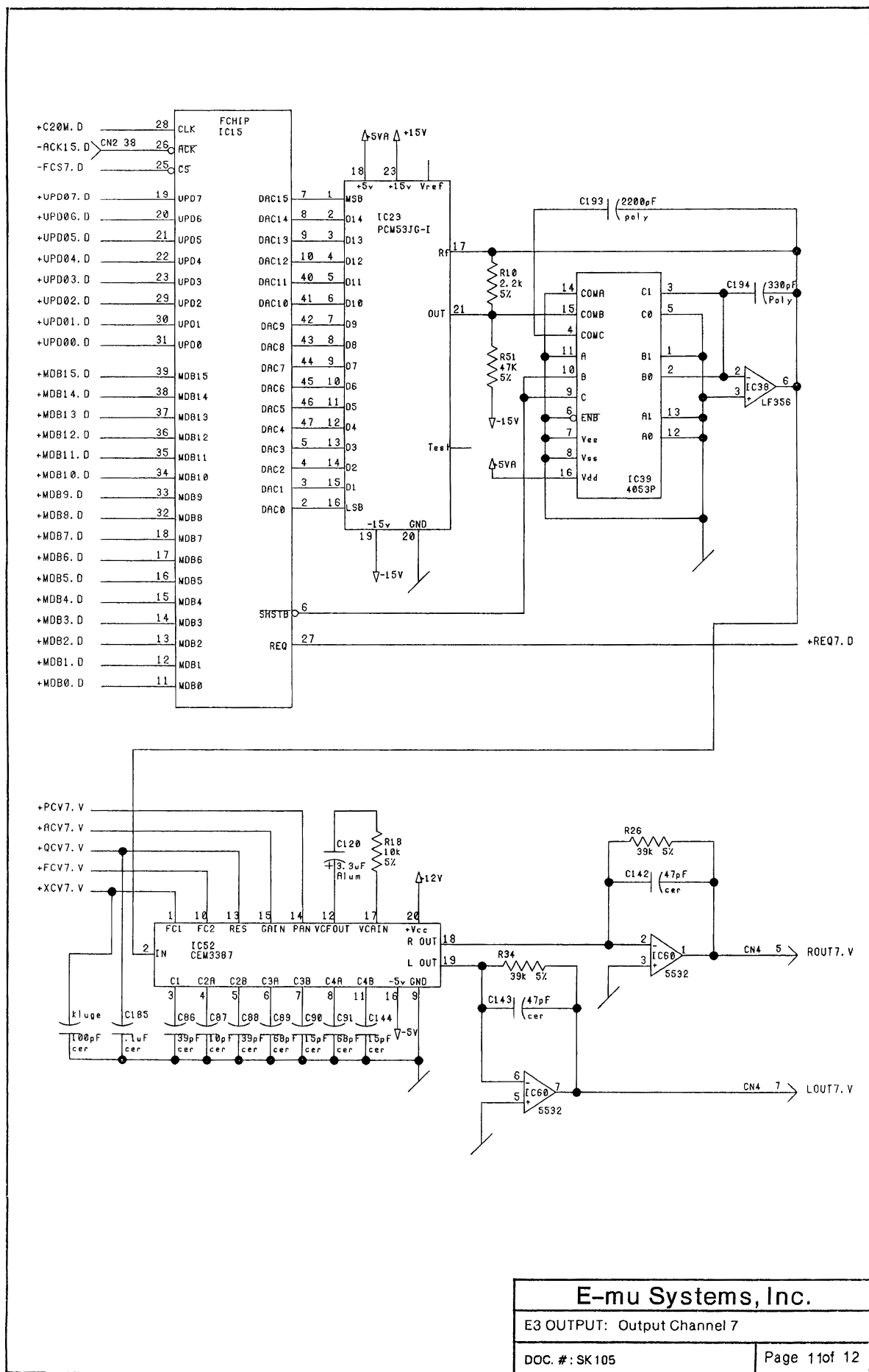
Output Board — SK105 sheet 11 of 12: Output: Output Channel 7.
