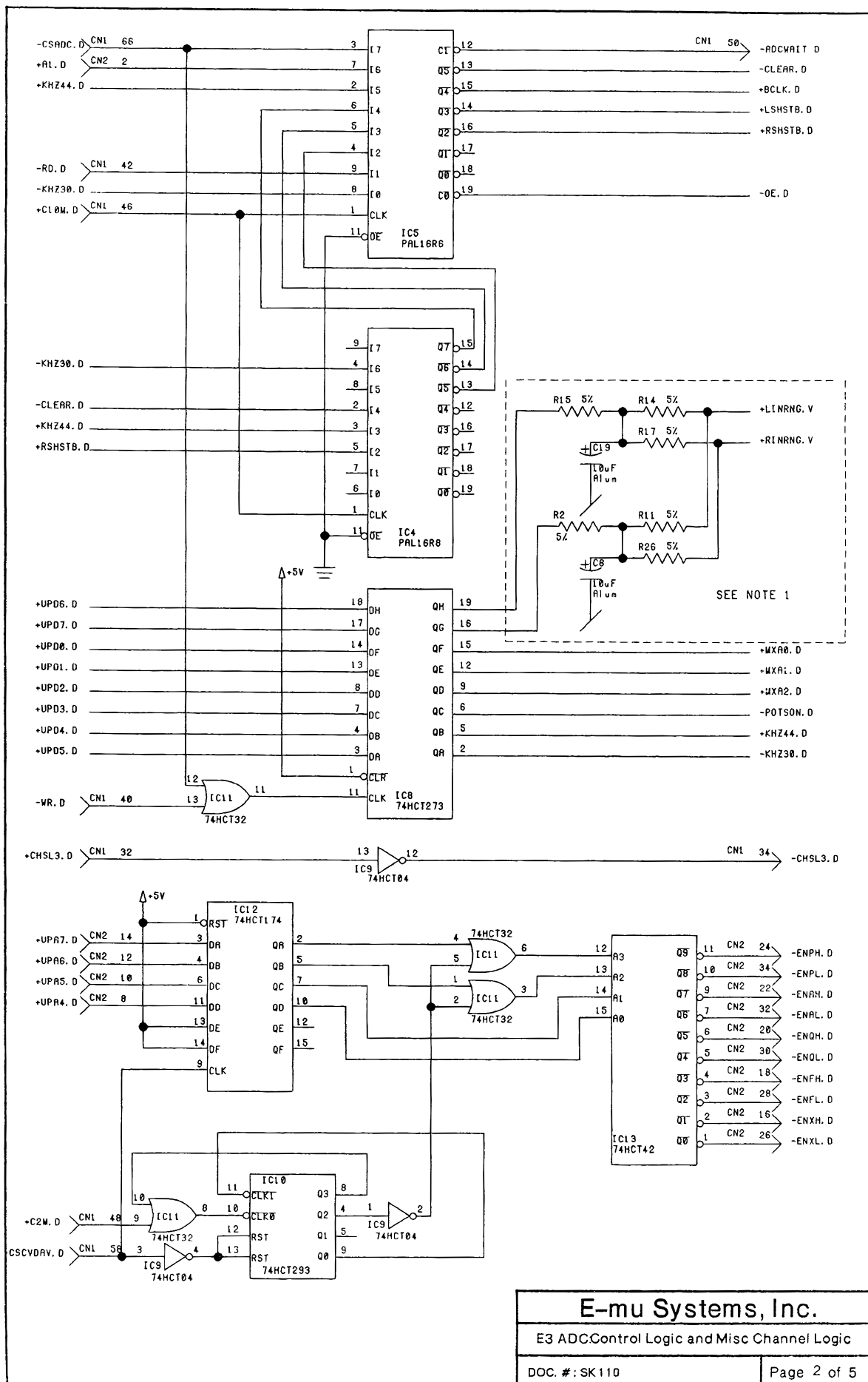
ADC Board — SK110 sheet 2 of 5: ADC: Control Logic and Misc Channel Logic.
