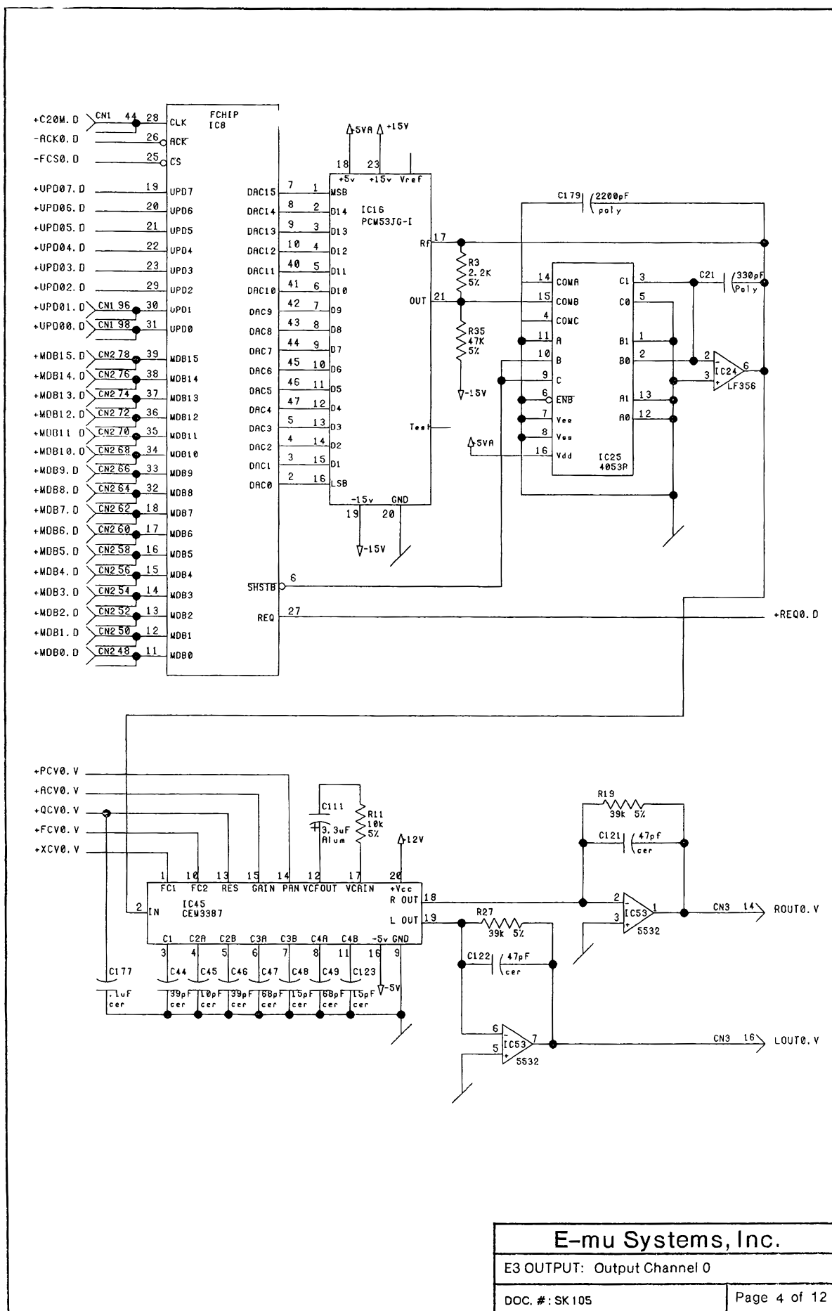
Output Board — SK105 sheet 4 of 12: Output: Output Channel 0.
