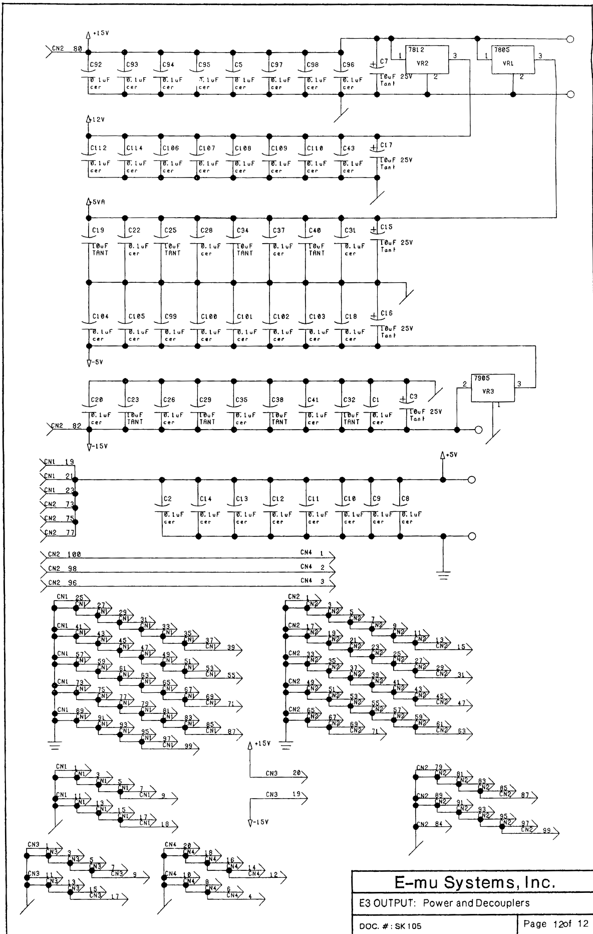
Output Board — SK105 sheet 12 of 12: Output: Power and Decouplers.
