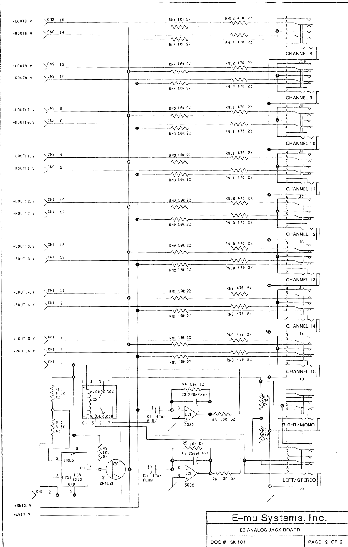
Analog Jack Board — SK107 sheet 2 of 2: Analog Jack Board.
