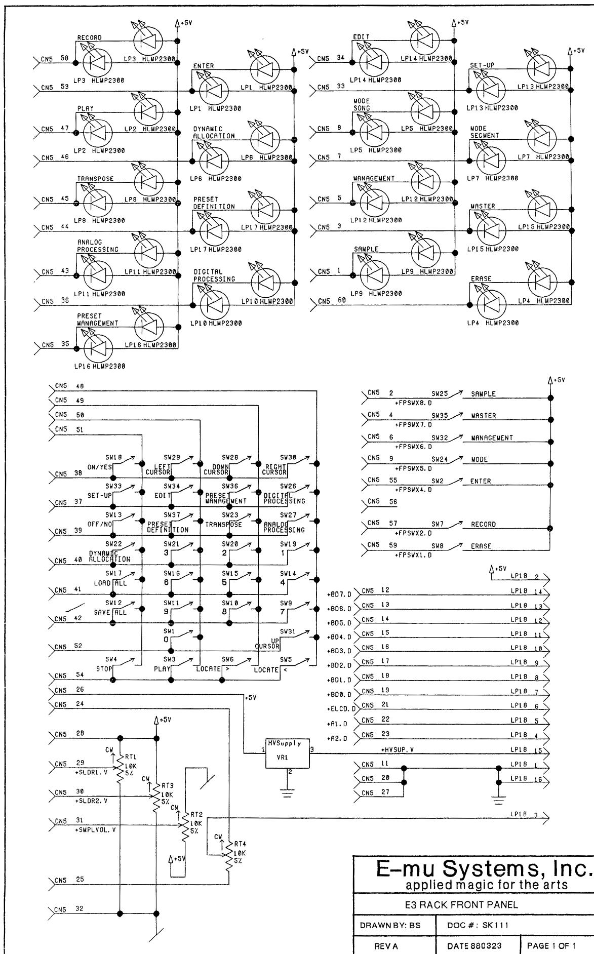
Rack Front Panel — SK111 sheet 1 of 1: E3 Rack Front Panel.
