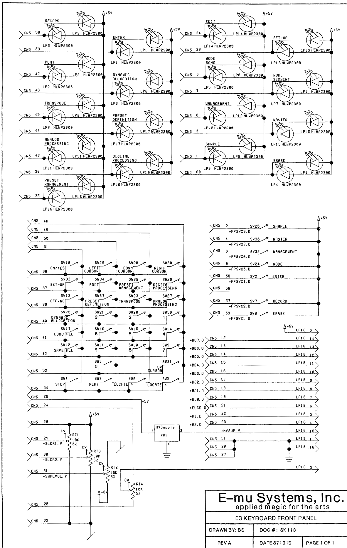
Keyboard Front Panel — SK113 sheet 1 of 1: E3 Keyboard Front Panel.
