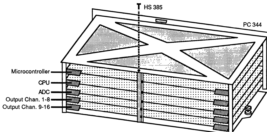
The PC 344 motherboard and card cage. Board order from top to bottom: Microcontroller, CPU, ADC, Output Chan. 1-8, Output Chan. 9-16.
