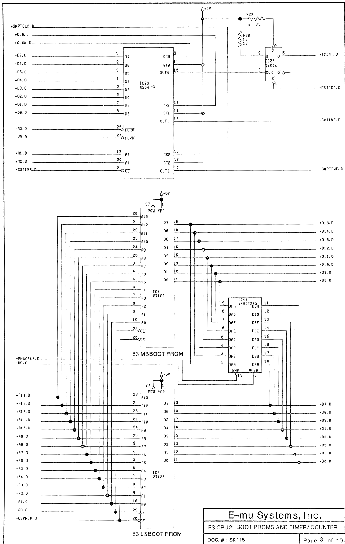
CPU Board (CPU2) — SK115 sheet 3 of 10: CPU2: Boot PROMs and Timer/Counter.
