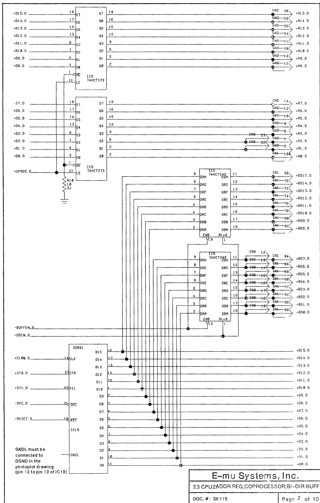
CPU Board (CPU2) — SK115 sheet 2 of 10: CPU2: Addr Reg, Coprocessor, Bi-Dir Buff.
