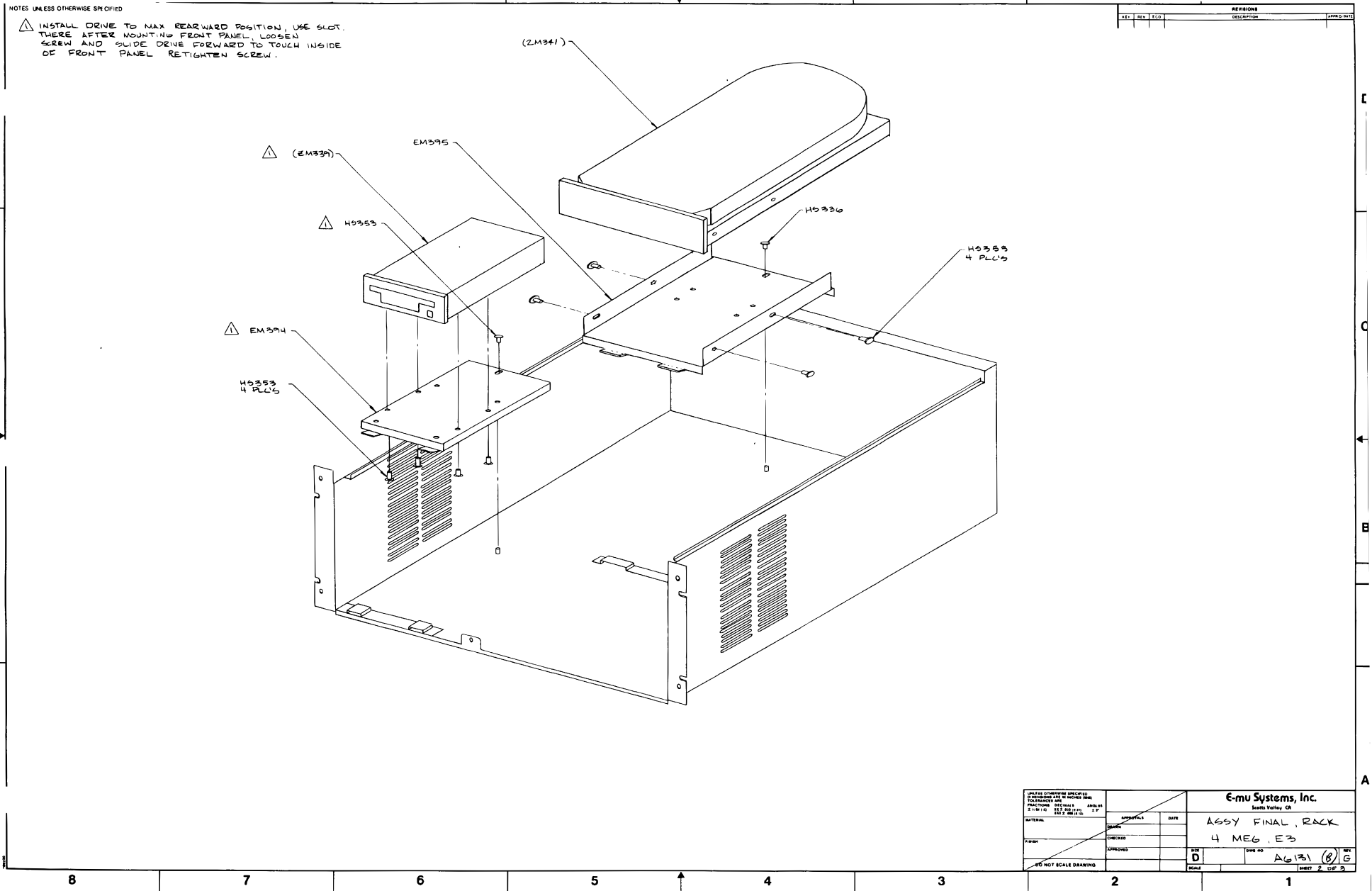
Drawing AG131, sheet 2 of 3 — Final assembly, rack 4 MEG E3, Rev G.
