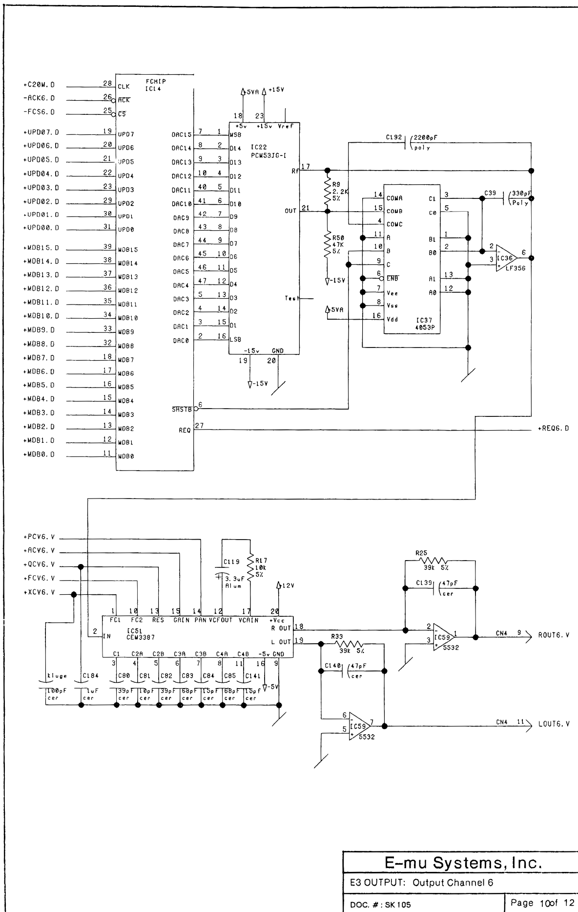
Output Board — SK105 sheet 10 of 12: Output: Output Channel 6.
