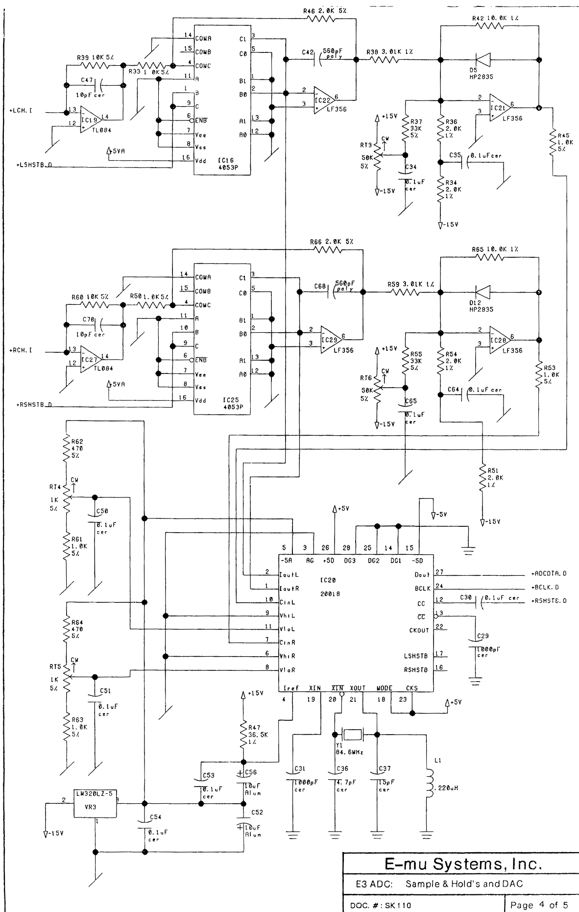
ADC Board — SK110 sheet 4 of 5: ADC: Sample & Holds and DAC.
