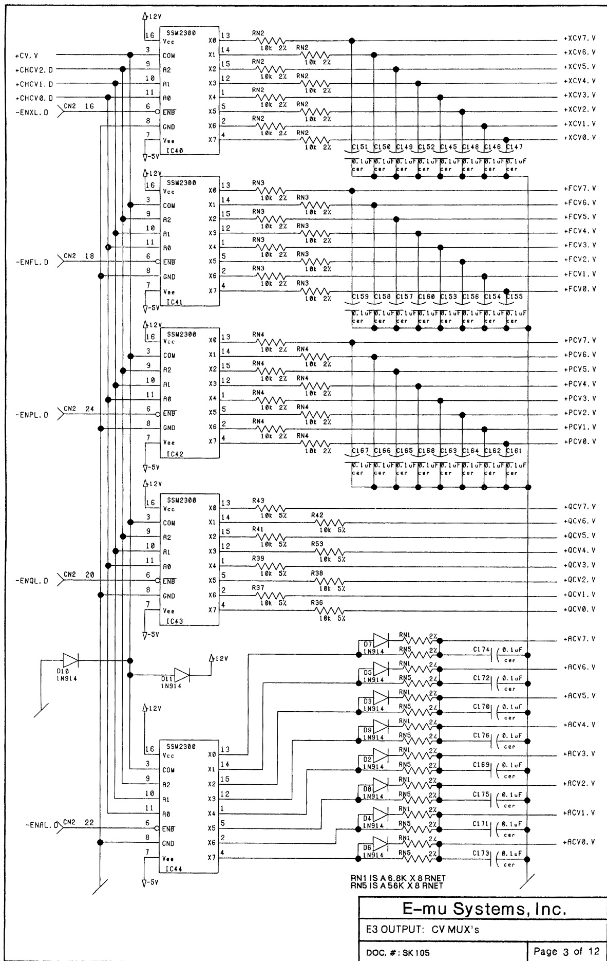
Output Board — SK105 sheet 3 of 12: Output: CV MUXes.
