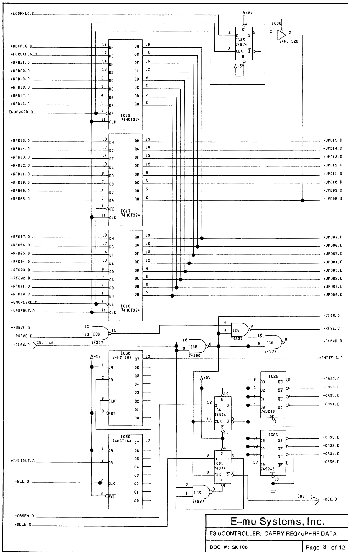
Microcontroller Board — SK106 sheet 3 of 12: uController: Carry Reg / uP+RF Data.
