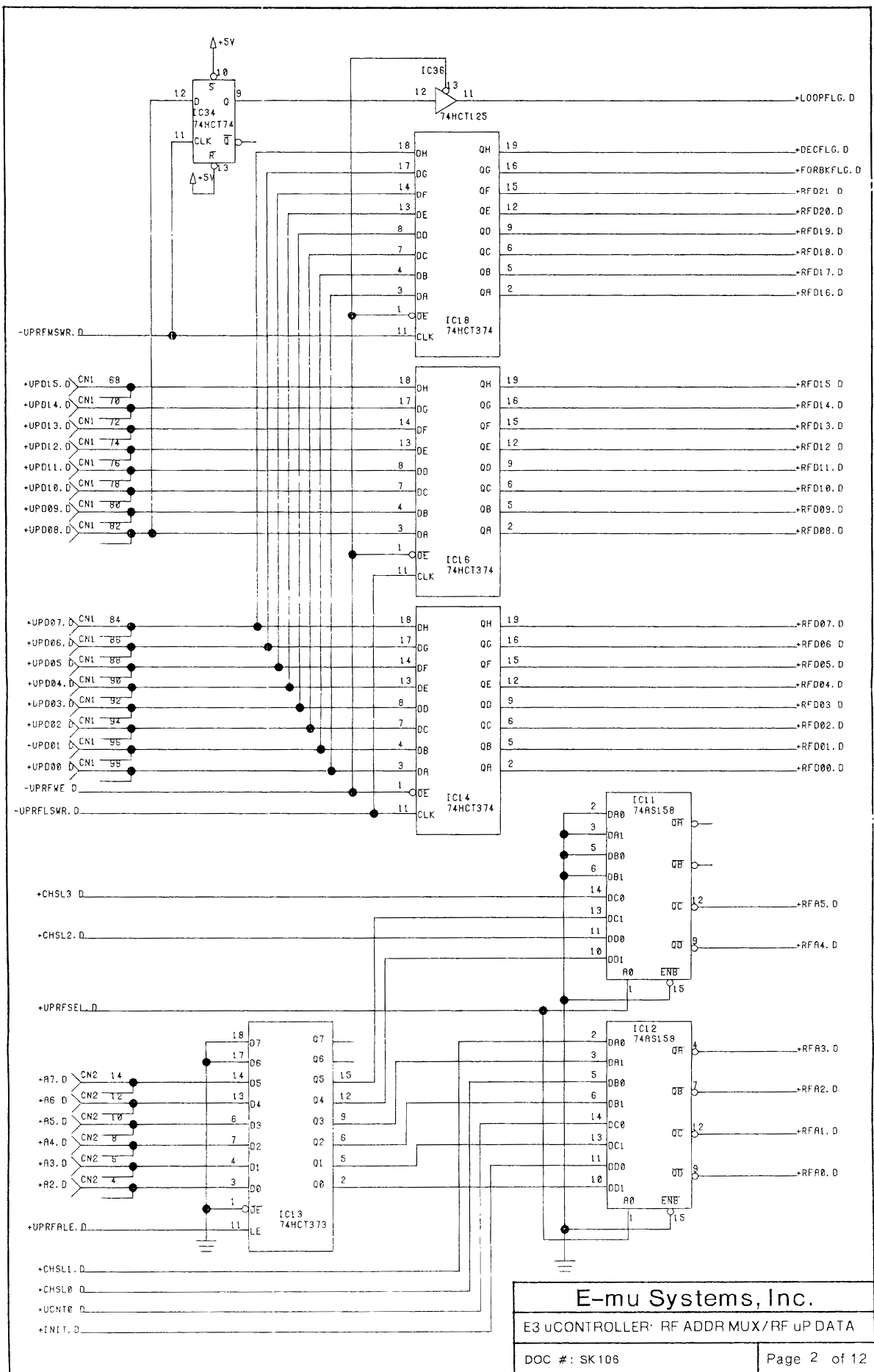
Microcontroller Board — SK106 sheet 2 of 12: uController: RF Addr Mux / RF uP Data.
