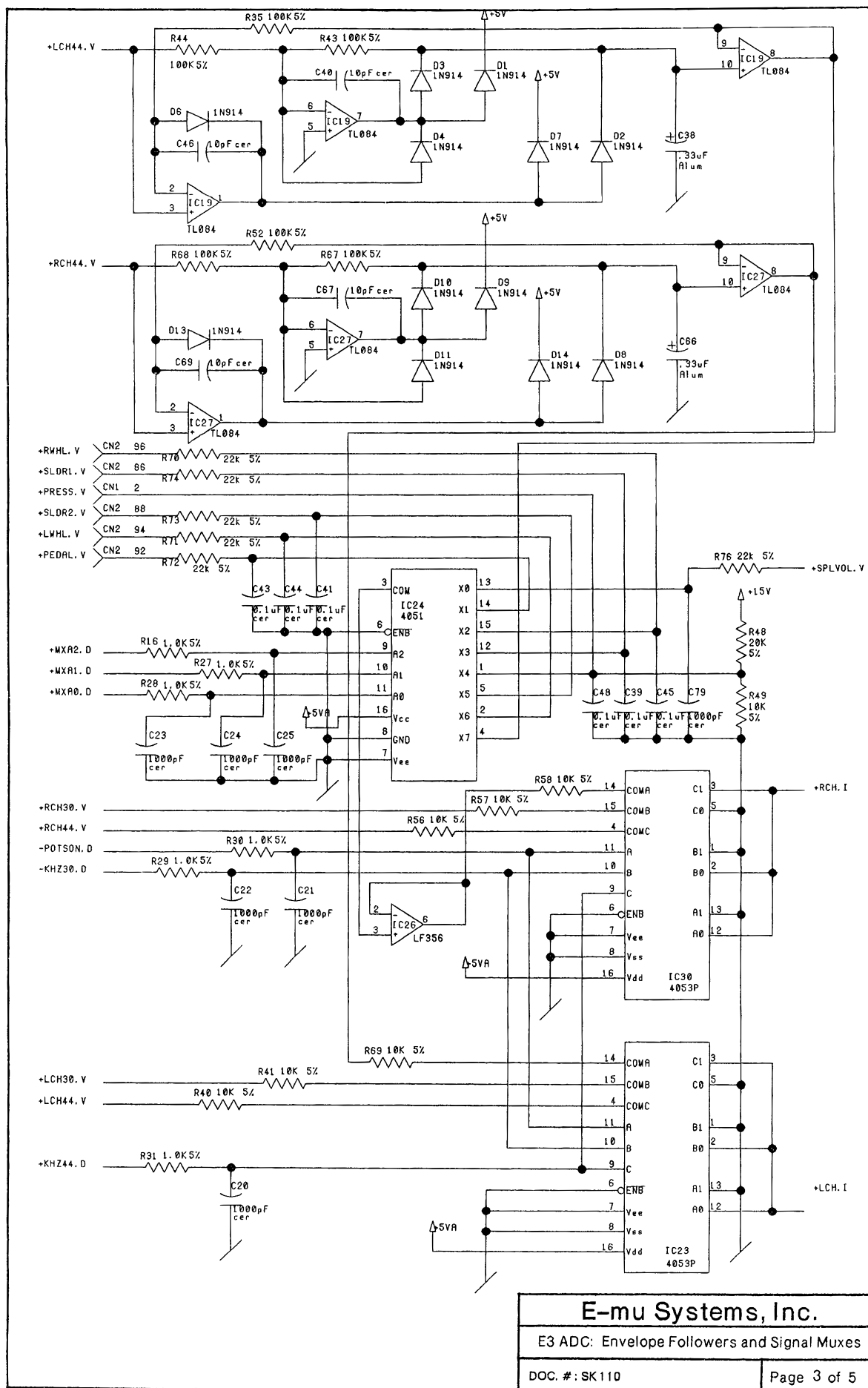
ADC Board — SK110 sheet 3 of 5: ADC: Envelope Followers and Signal Muxes.
