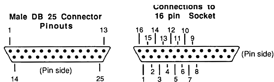
Monitor cable: male DB25 connector pinouts (pin side) and connections to the 16-pin socket.
