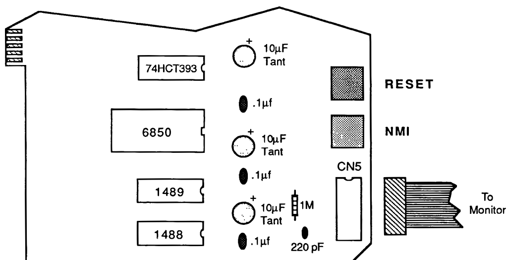
Debug board parts layout: 74HCT393, 6850 ACIA, 1489 RS-232 receiver, 1488 RS-232 driver, three 10 µF tantalum and three 0.1 µF capacitors, 1M resistor, 220 pF capacitor, RESET and NMI buttons, and the 16-pin socket CN5 with the ribbon cable to the monitor.
