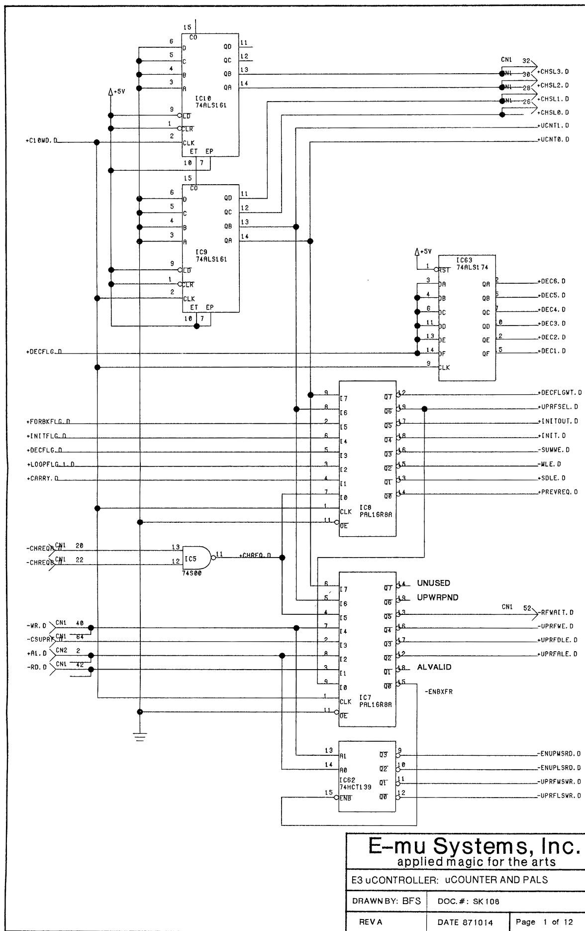
Microcontroller Board — SK106 sheet 1 of 12: uController: uCounter and PALS.
