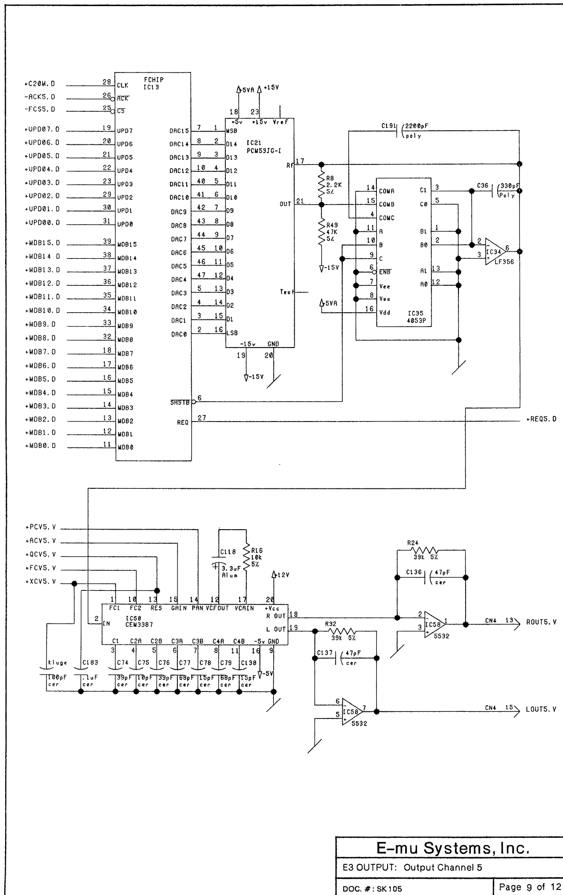
Output Board — SK105 sheet 9 of 12: Output: Output Channel 5.
