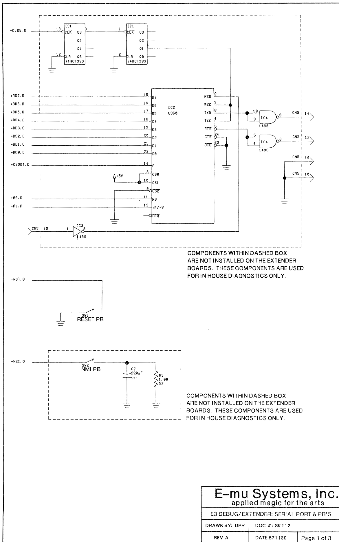
Debug/Extender Board — SK112 sheet 1 of 3: Debug/Extender: Serial Port & PB's.
